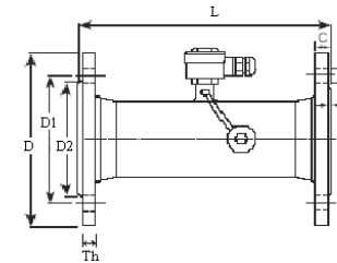
Standard-type Flow-cell Transducer
