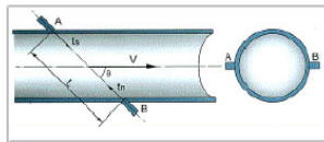
Z-method for large pipe
