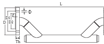
Pi-type Flow-cell Transducer
